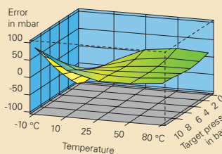
Standard Transmitter
