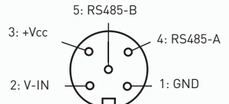
M12/5-pin (f)
