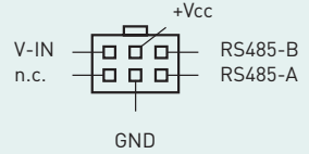
Molex socket 6-pin (f)
