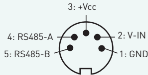
Binder Series 723/5-pin (m)
